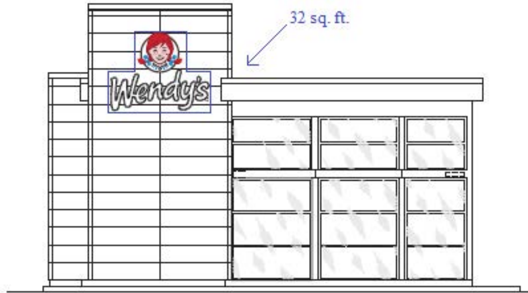
FRONT ELEVATION SCALE 3/32" : 1'
